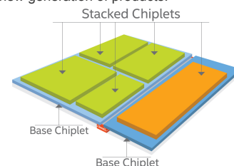
"Foveros" 3D packaging technology
